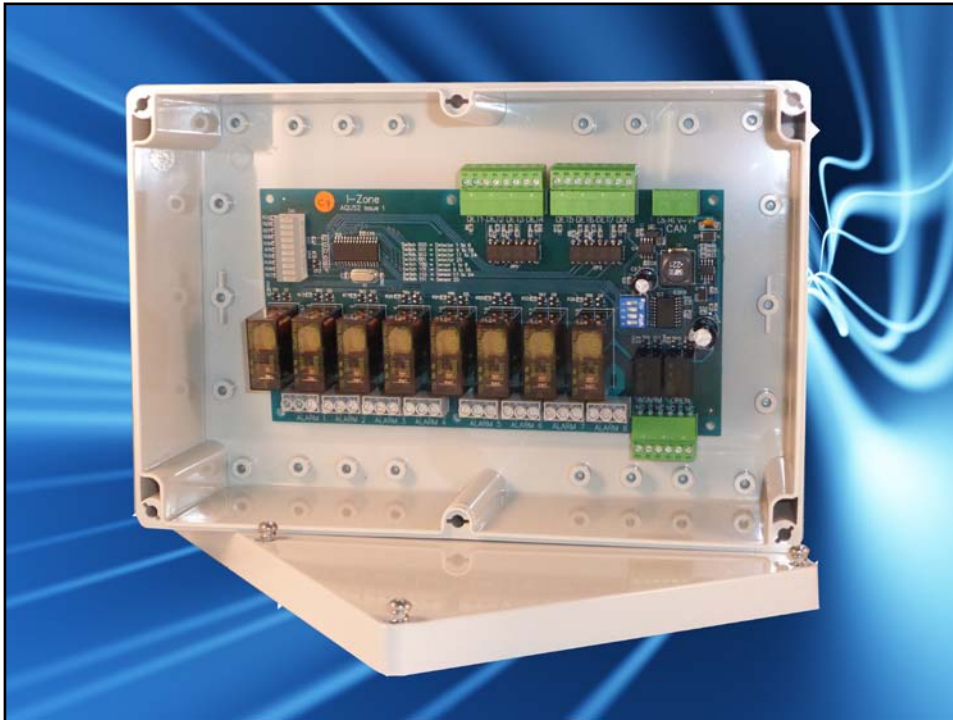
8 Input/Output Relay Pack
